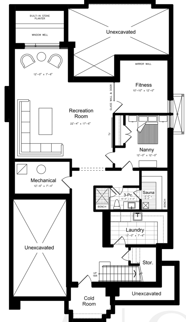
LOWER LEVEL APPROX. 1648 SQ FT
