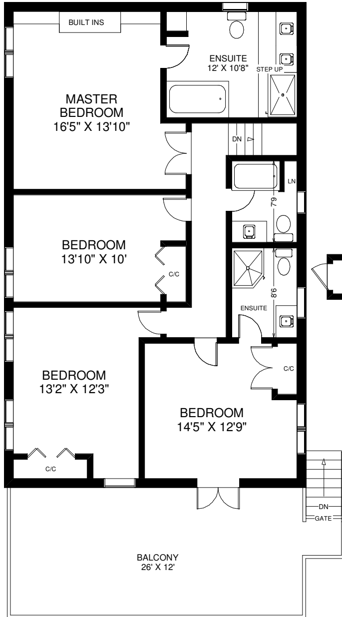
SECOND FLOOR APPROXIMATELY 1,300 SQ FT
